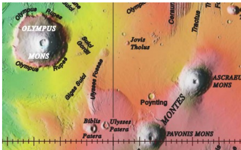
Illustration 8: Topographic map for north of the equator (approx. 2S-28N, 130W-100W). Image credit: USGS
